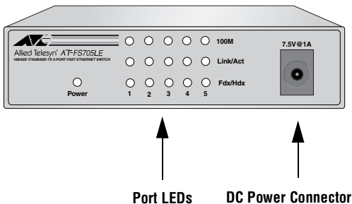
Figure 2 Front Panel
